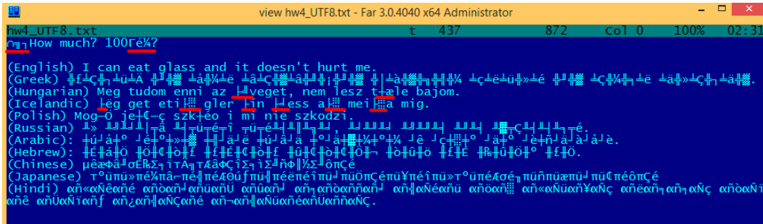
Рис. 5.2: FAR: UTF-8
